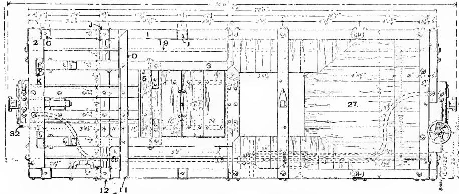
Fig. 326. Plan of Framing and Hopper. ORE-CAR BODY. DULUTH & IRON RANGE RAILROAD. Length, 22 ft. Capacity, 48,000 lbs.
